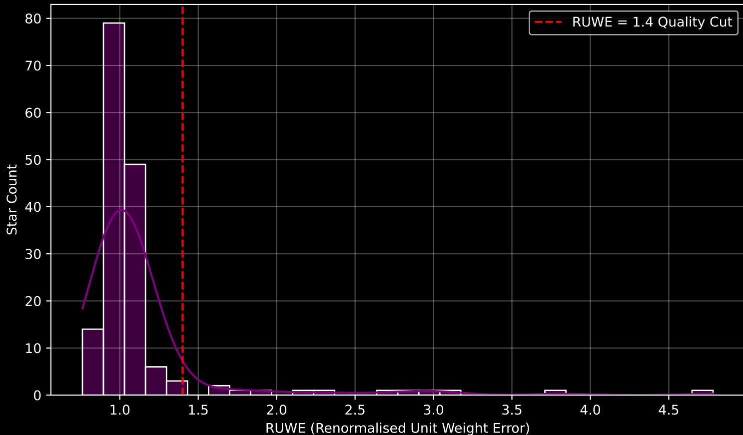
GAPOGEE DR17 Field [090+30] RUWE Distribution (n= 163)
