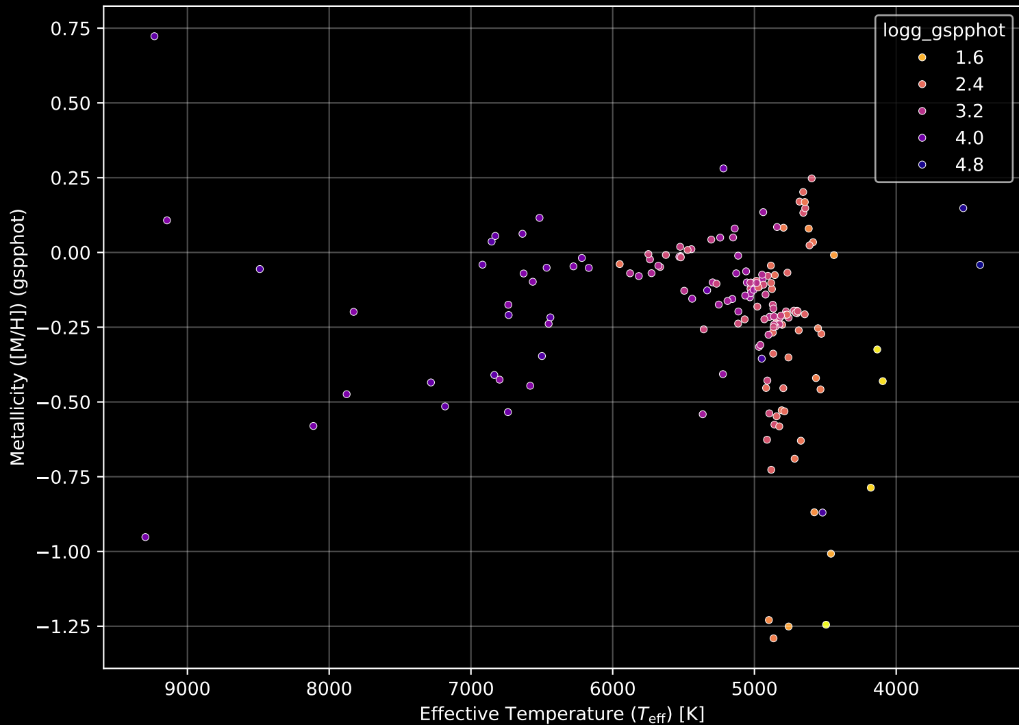
APOGEE DR17 Field: [090+30] Stellar Population Parameters (n= 166)
