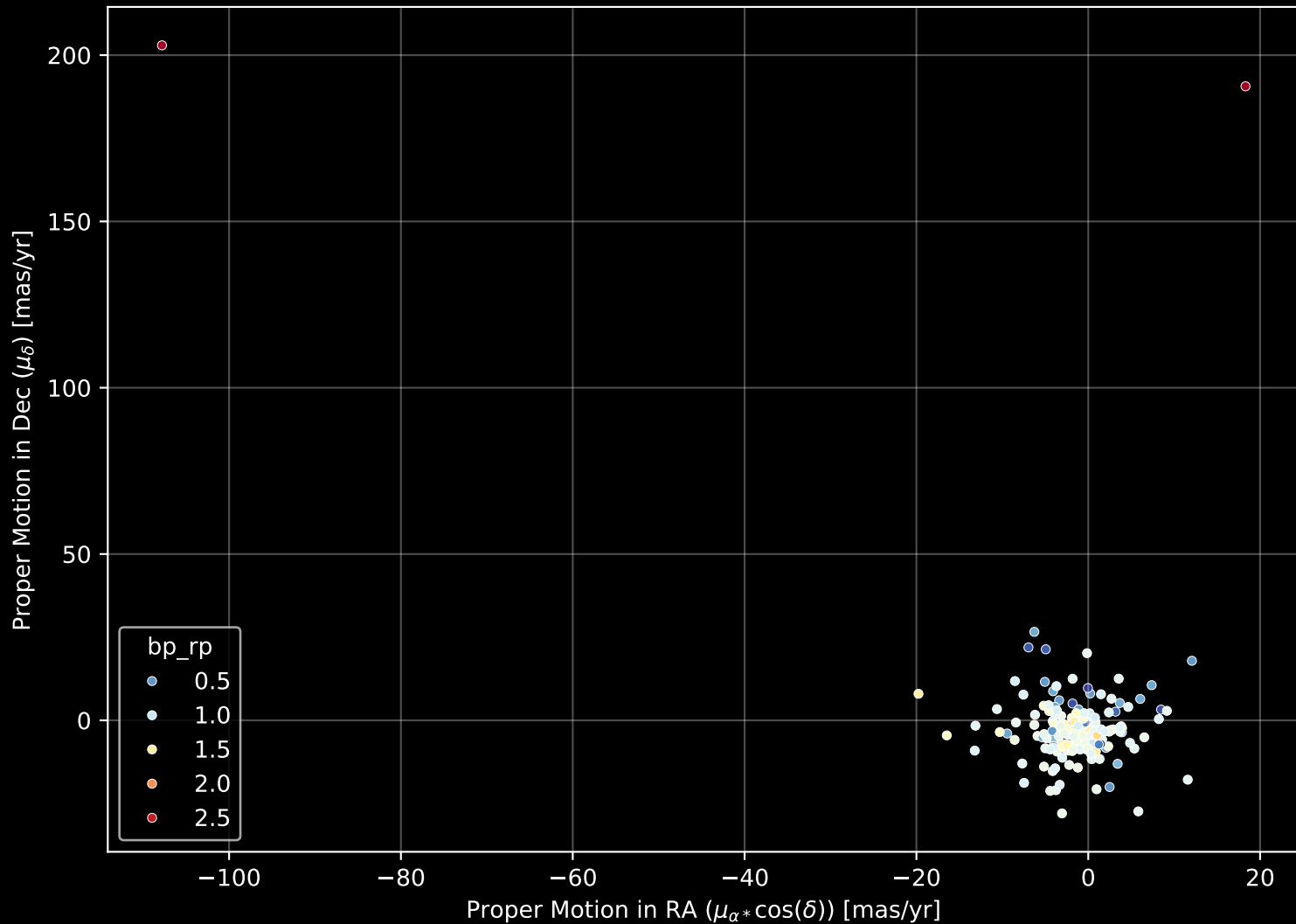
APOGEE DR17 Field: [090+30] Proper Motion Diagram (n= 166)
