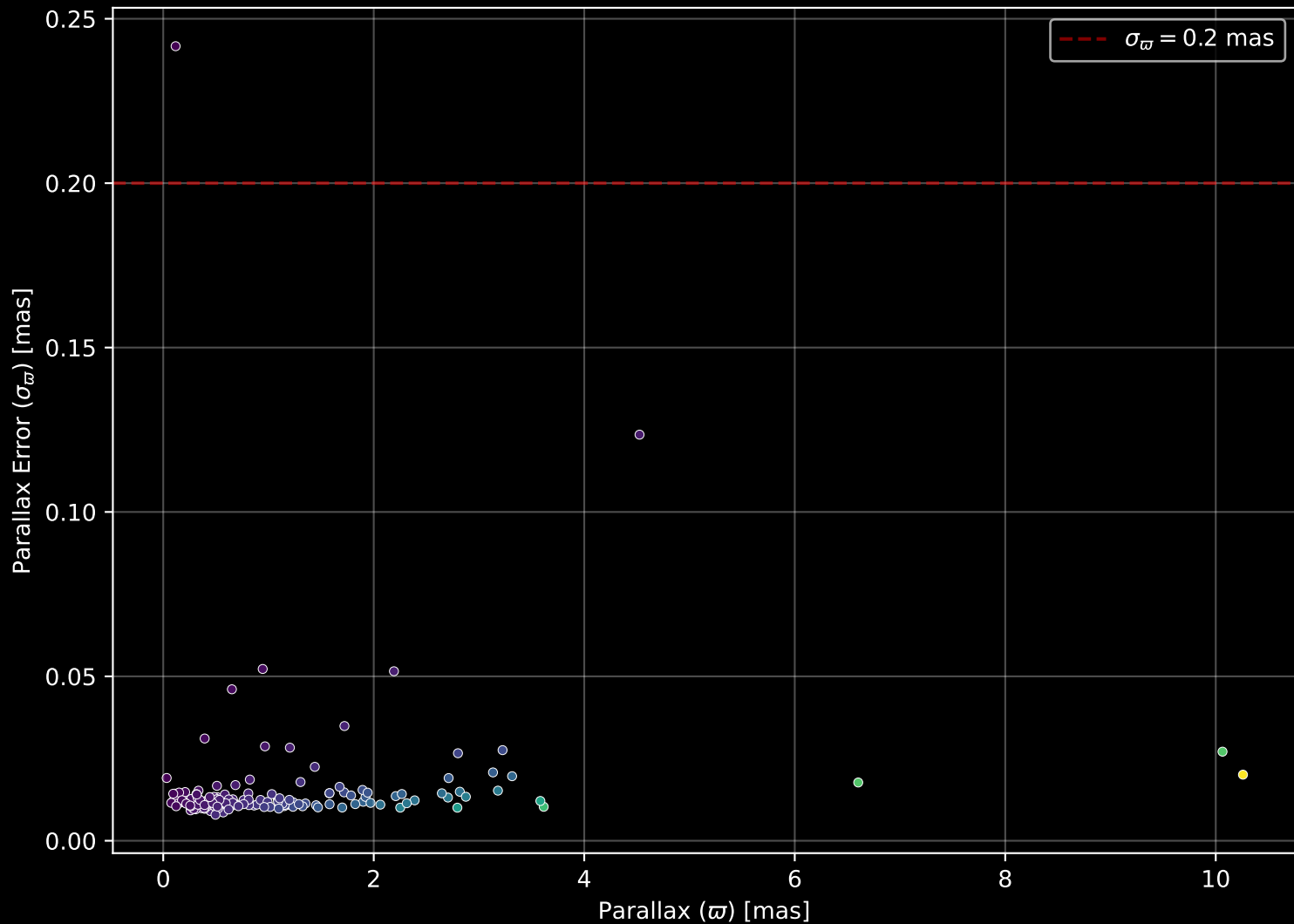
APOGEE DR17 Field: [090+30] Parallax Quality (n= 166)
