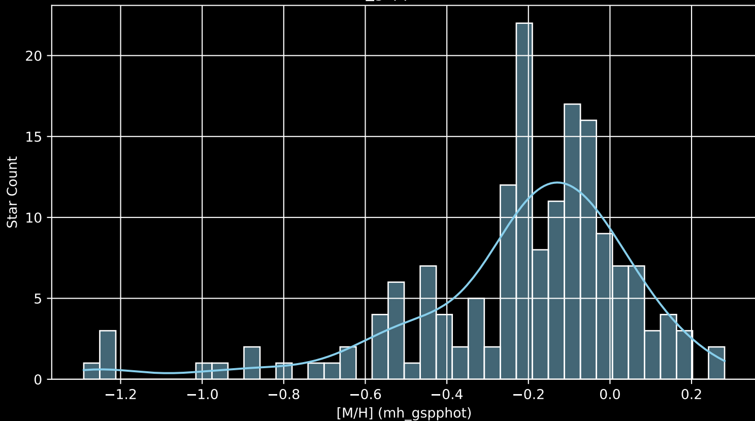
APOGEE DR17 Field: [090+30 [M/H] (mh_gspphot) (n= 165)
